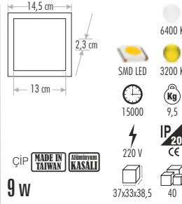
CT-5137 5" PANEL LED ARMATÜR
