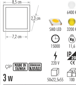
CT-5135 3" PANEL LED ARMATÜR
