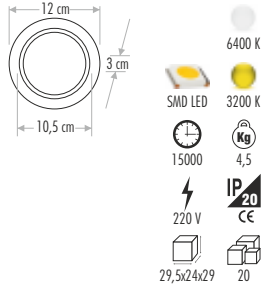
CT-5196 GOLD LED PANEL ARMATÜR
