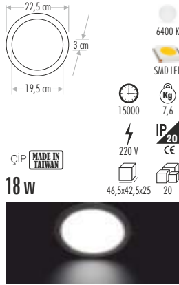
CT-5122 10" PANEL LED ARMATÜR
