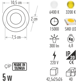
CT-5120 OKYANUS LED PANEL ARMATÜR 40,00 ₺
