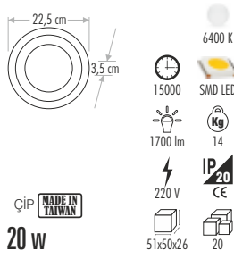
CT-5159 OKYANUS LED PANEL ARMATÜR 130,00 ₺
