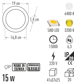
CT-5149 8" PANEL LED ARMATÜR
