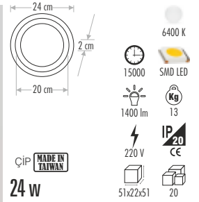
CT-5153 OKYANUS LED PANEL ARMATÜR 110,00 ₺
