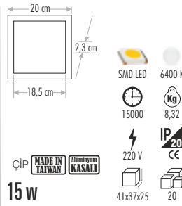
CT-5139 8" PANEL LED ARMATÜR
