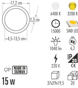
CT-5657 PLUS LED PANEL ARMATÜR
