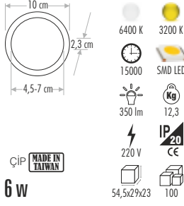
CT-5655 PLUS LED PANEL ARMATÜR
