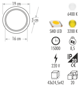
CT-5188 GOLD LED PANEL ARMATÜR
