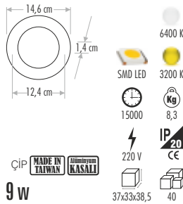
CT-5147 5" PANEL LED ARMATÜR
