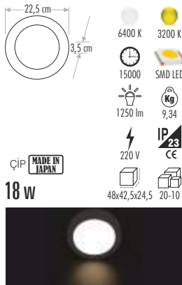
CT-5273 S 8" PANEL
