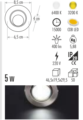
CT-5252 2" AKİK SATIN GÖVDE 26,00 ₺
